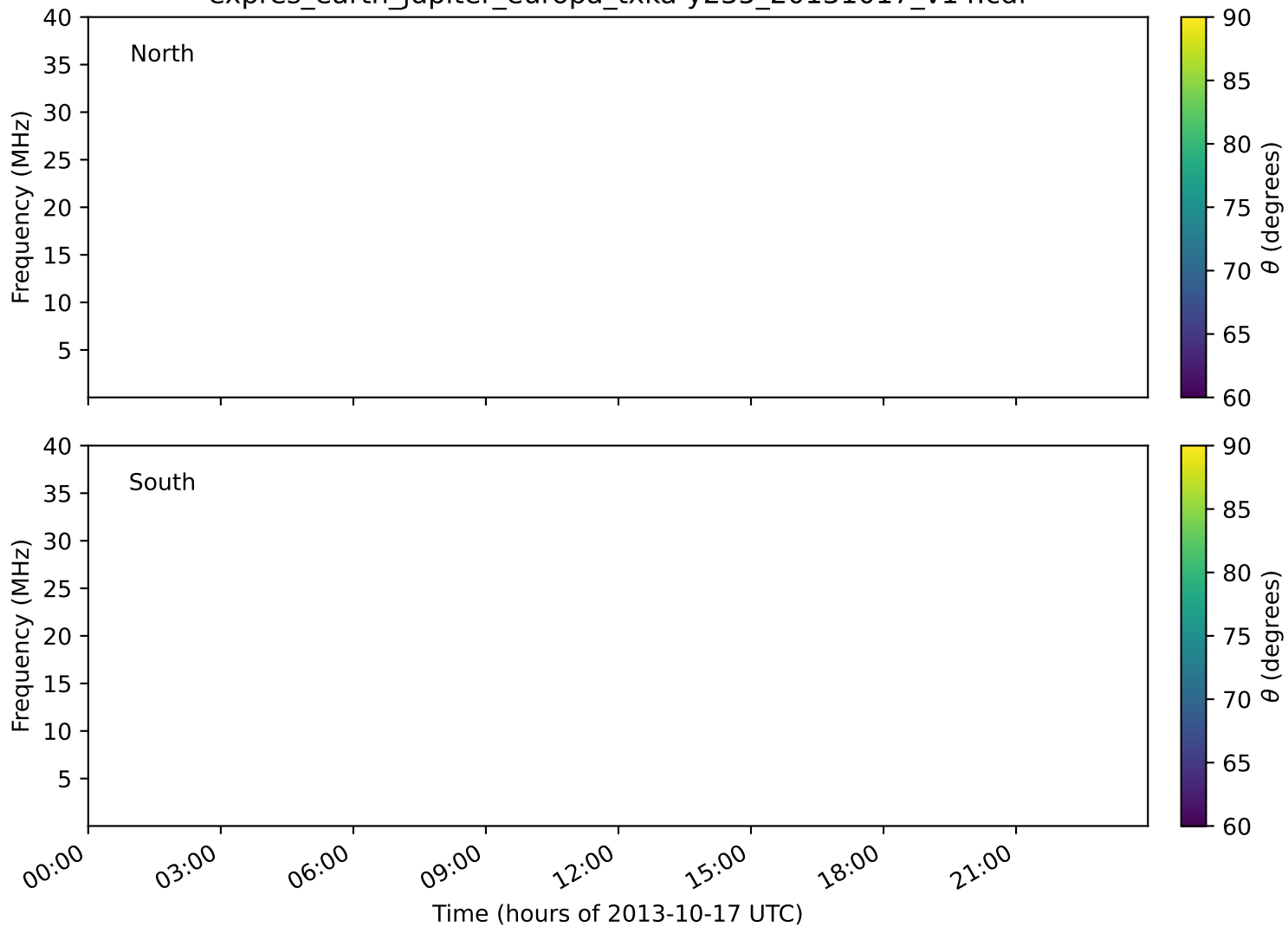
expres_earth_jupiter_europa_txka-y235_20131017_v14.cdf
