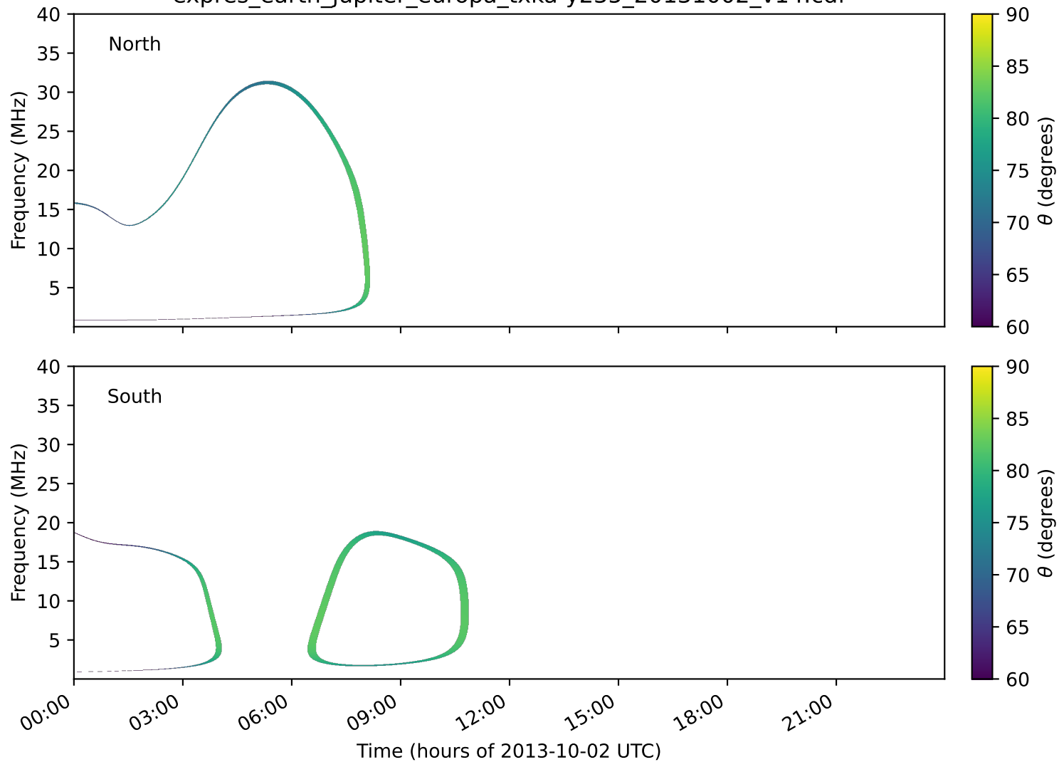
expres_earth_jupiter_europa_txka-y235_20131002_v14.cdf
