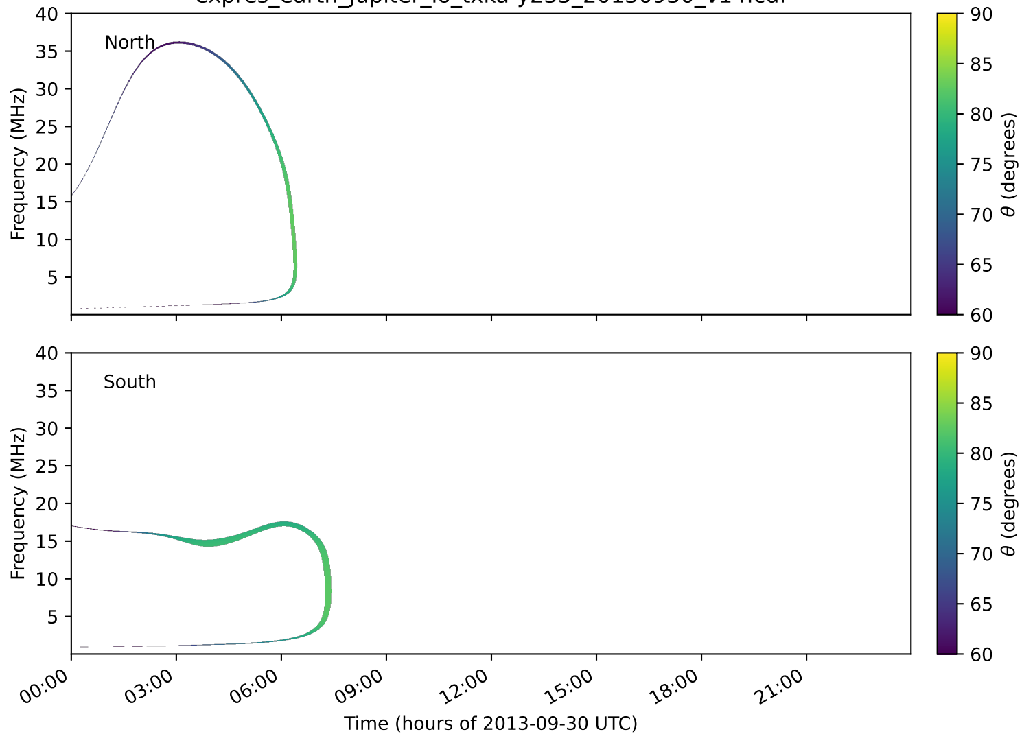
expres_earth_jupiter_io_txka-y235_20130930_v14.cdf
