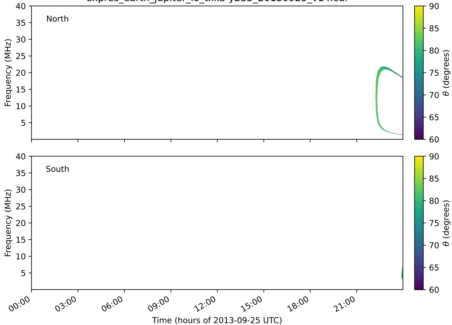
expres_earth_jupiter_io_txka-y235_20130925_v14.cdf
