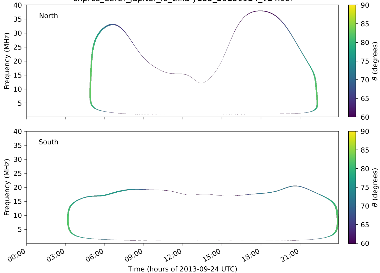
expres_earth_jupiter_io_txka-y235_20130924_v14.cdf
