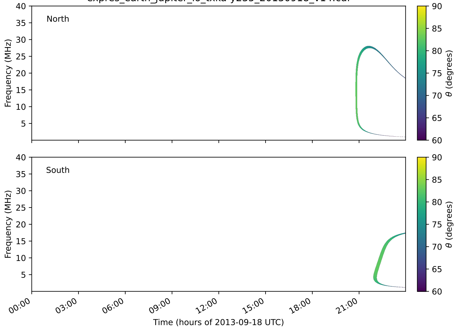
expres_earth_jupiter_io_txka-y235_20130918_v14.cdf
