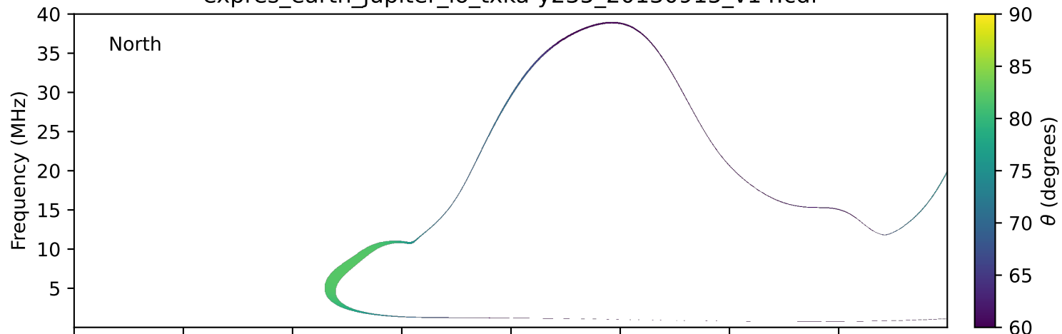
expres_earth_jupiter_io_txka-y235_20130915_v14.cdf
