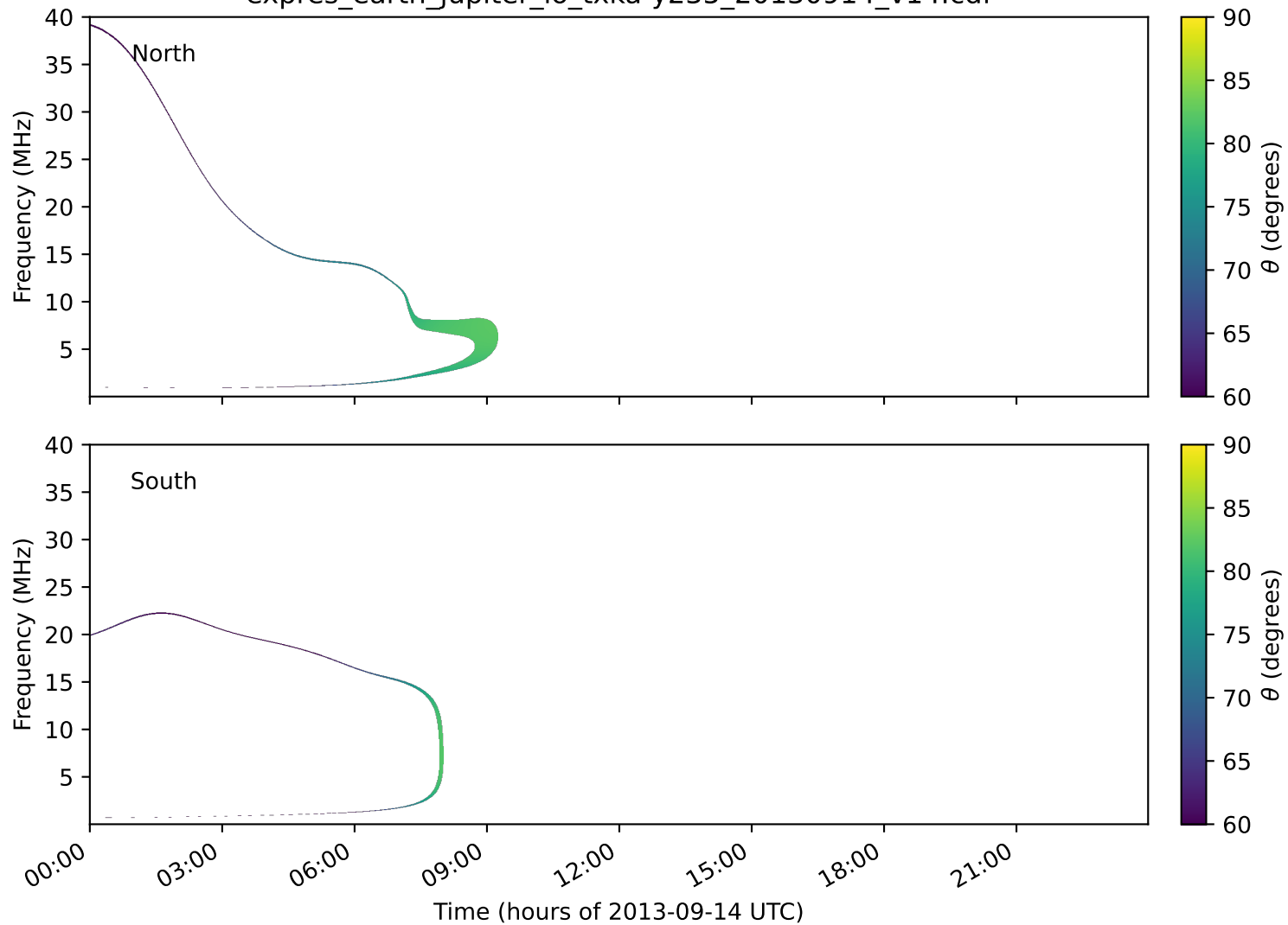
expres_earth_jupiter_io_txka-y235_20130914_v14.cdf
