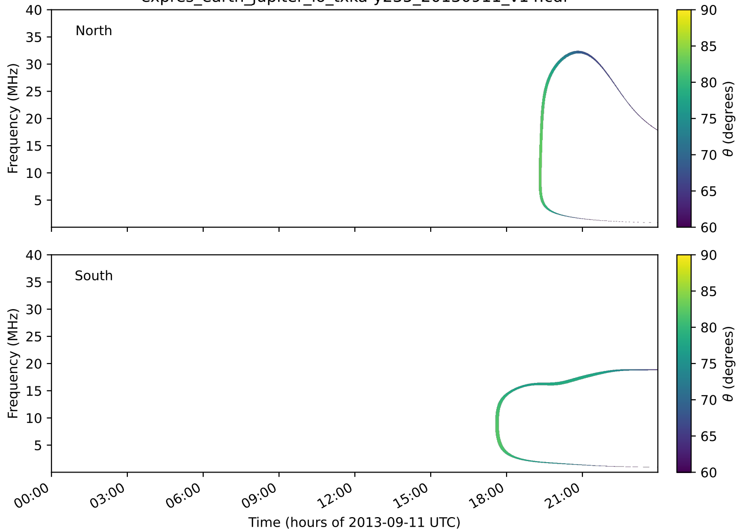
expres_earth_jupiter_io_txka-y235_20130911_v14.cdf
