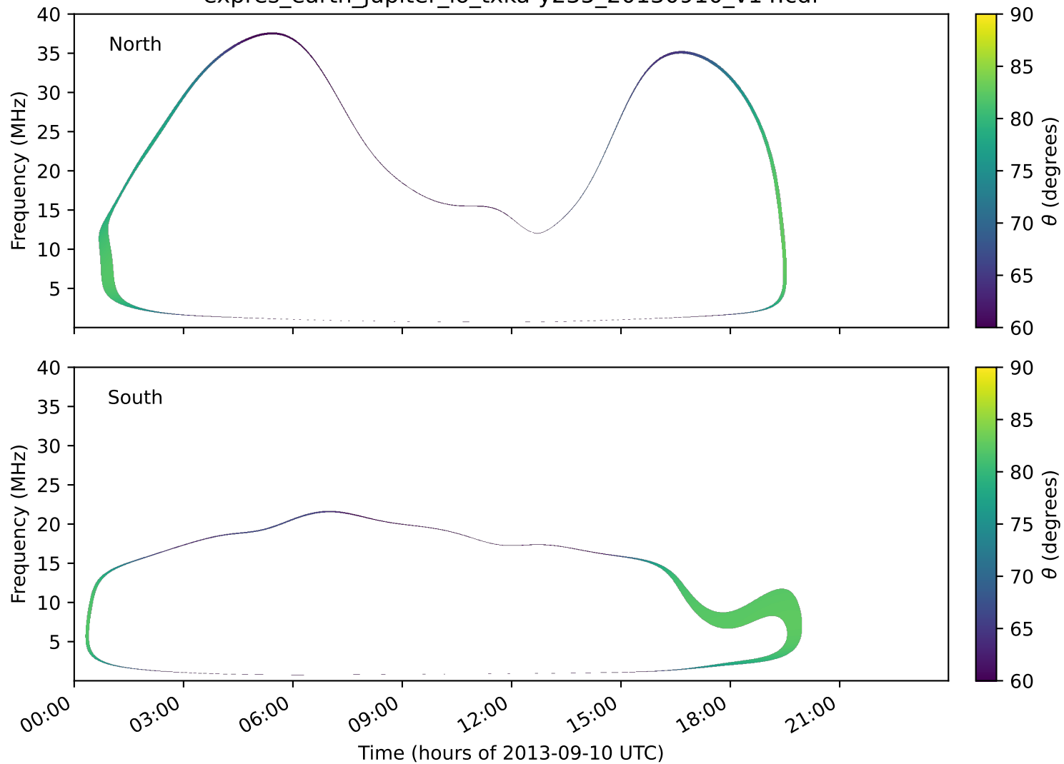
expres_earth_jupiter_io_txka-y235_20130910_v14.cdf
