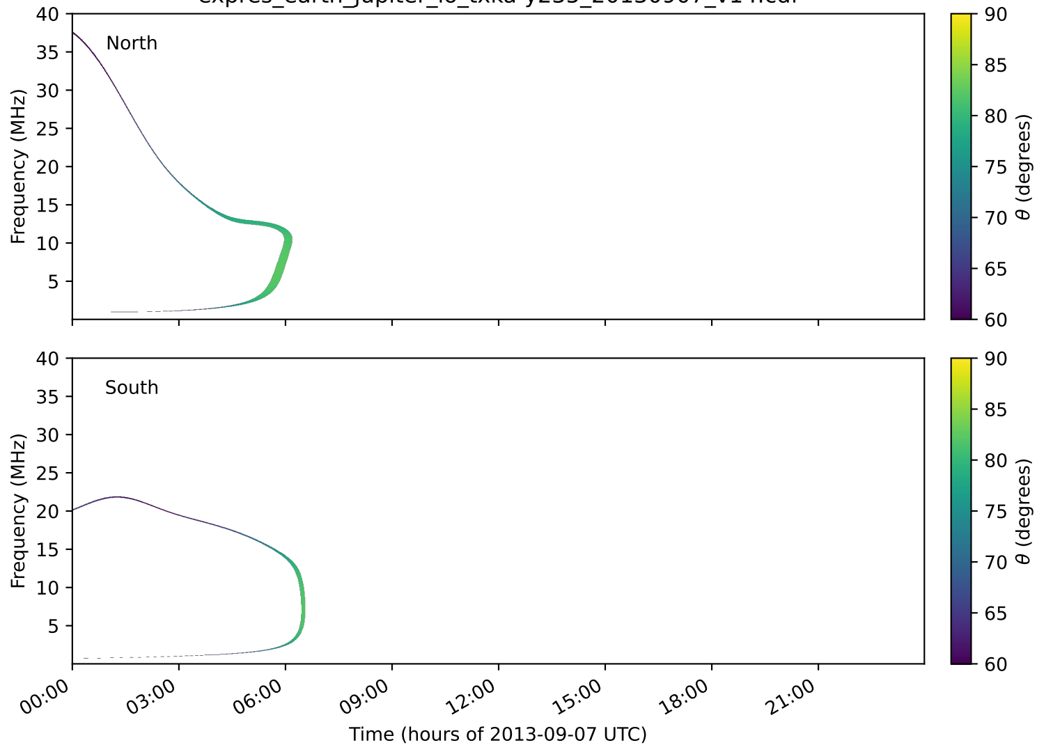
expres_earth_jupiter_io_txka-y235_20130907_v14.cdf
