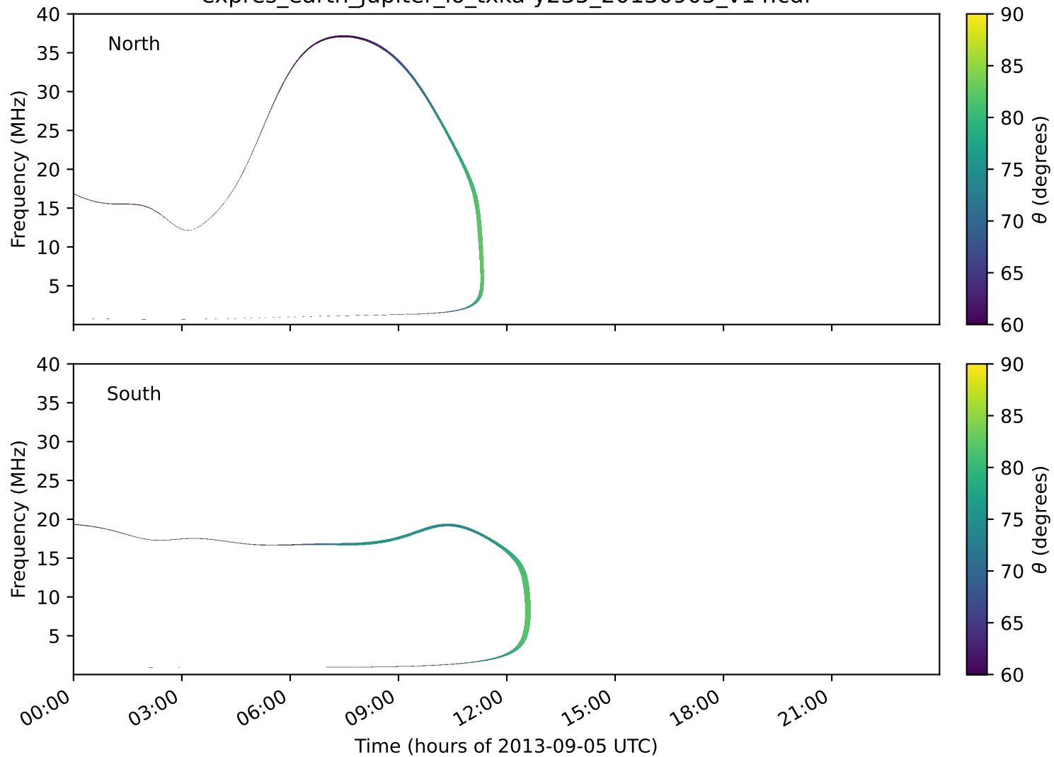
expres_earth_jupiter_io_txka-y235_20130905_v14.cdf
