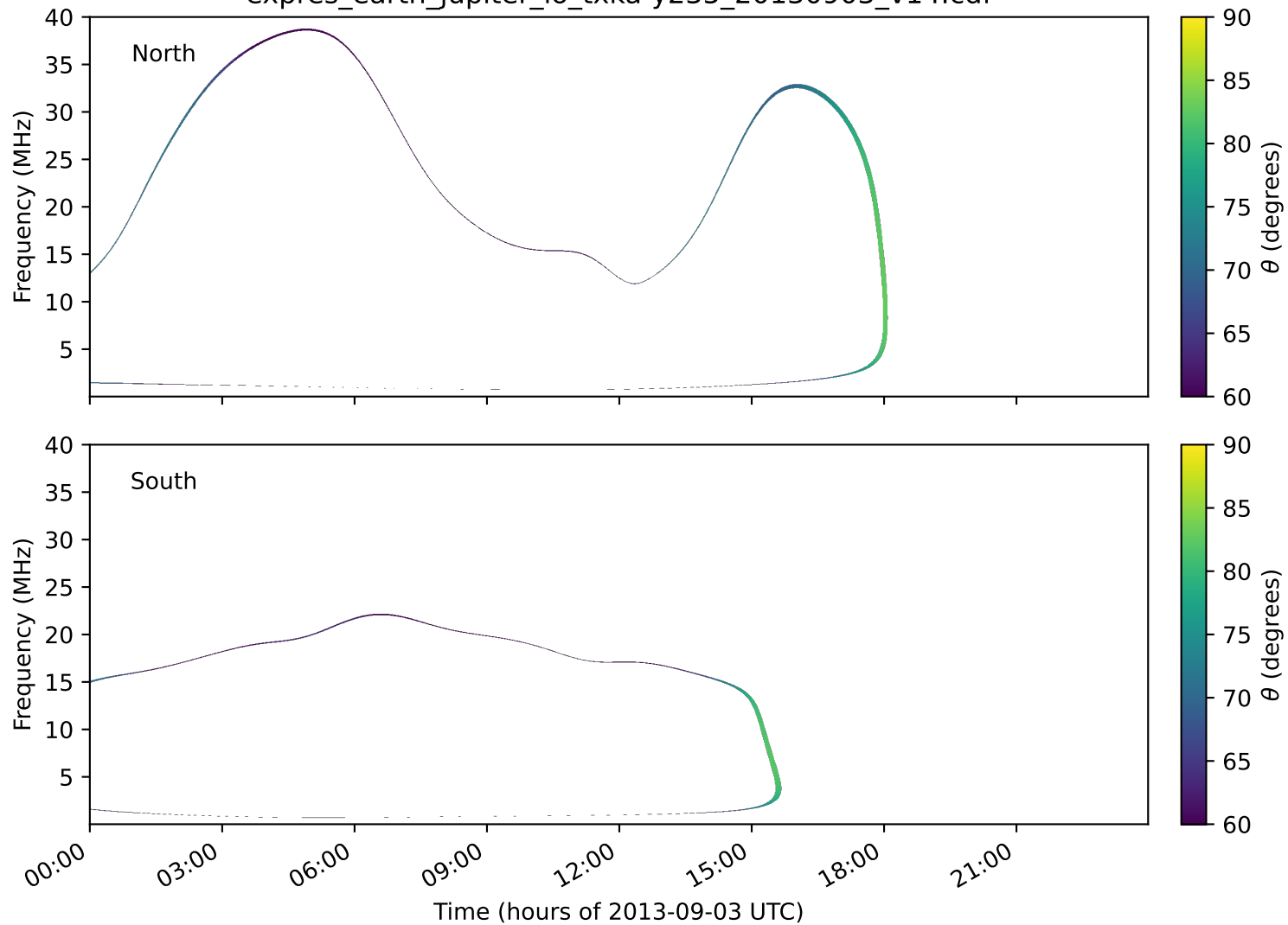
expres_earth_jupiter_io_txka-y235_20130903_v14.cdf
