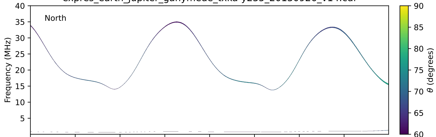
expres_earth_jupiter_ganymede_txka-y235_20130926_v14.cdf
