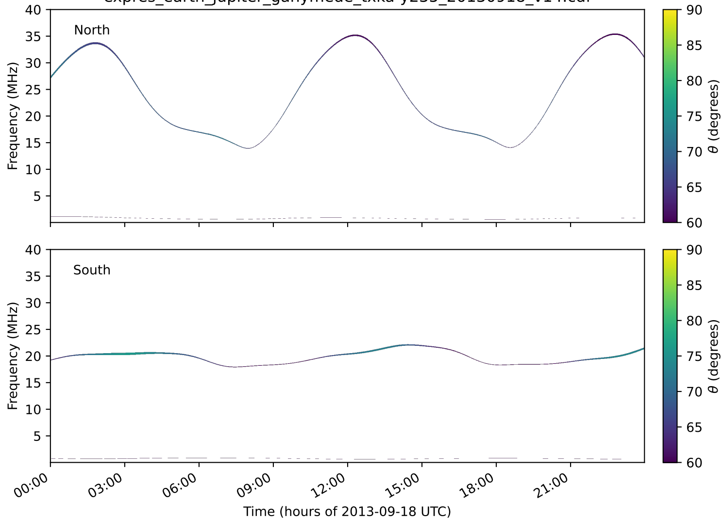
expres_earth_jupiter_ganymede_txka-y235_20130918_v14.cdf
