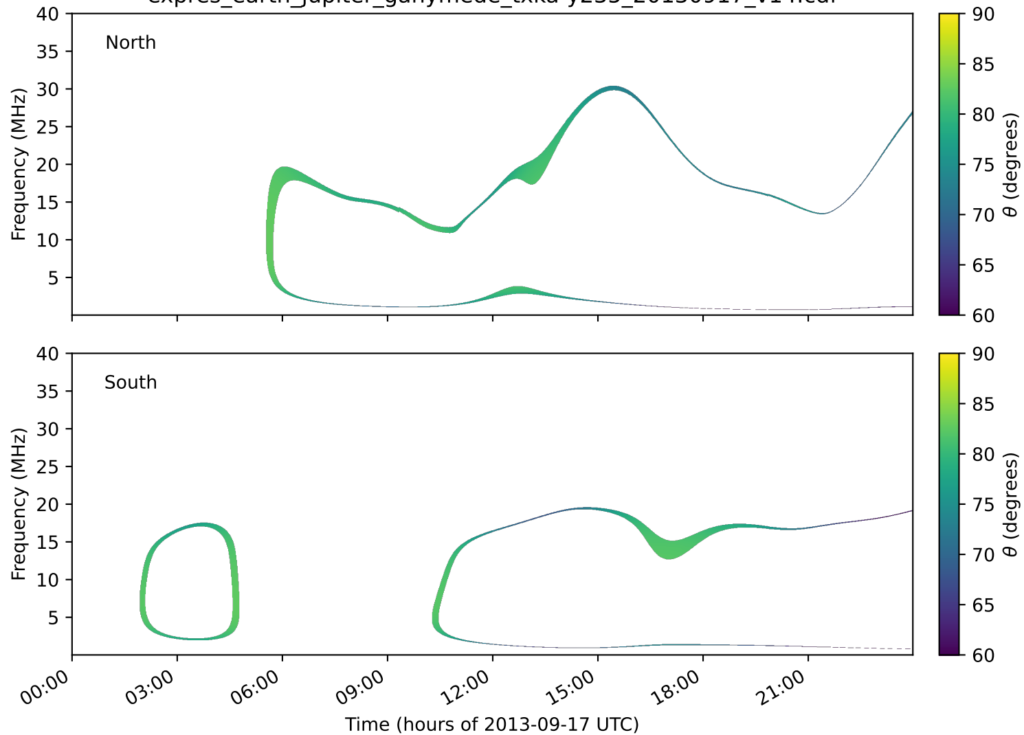
expres_earth_jupiter_ganymede_txka-y235_20130917_v14.cdf
