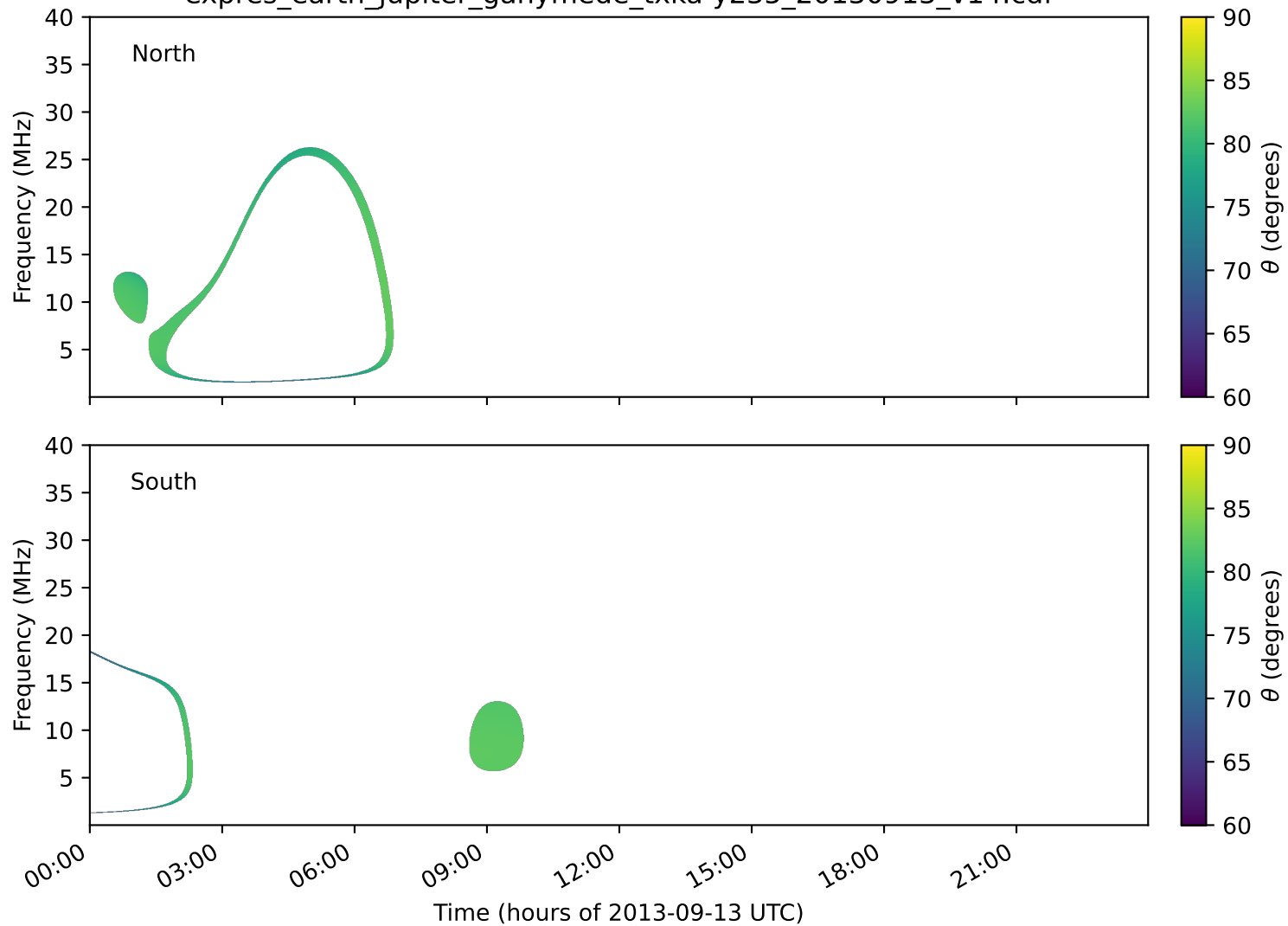
expres_earth_jupiter_ganymede_txka-y235_20130913_v14.cdf
