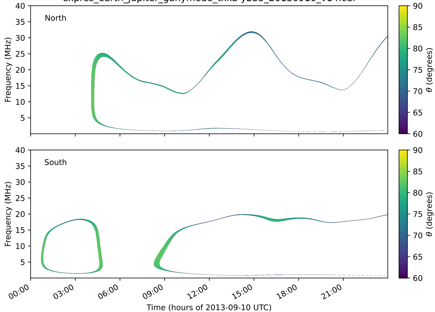
expres_earth_jupiter_ganymede_txka-y235_20130910_v14.cdf
