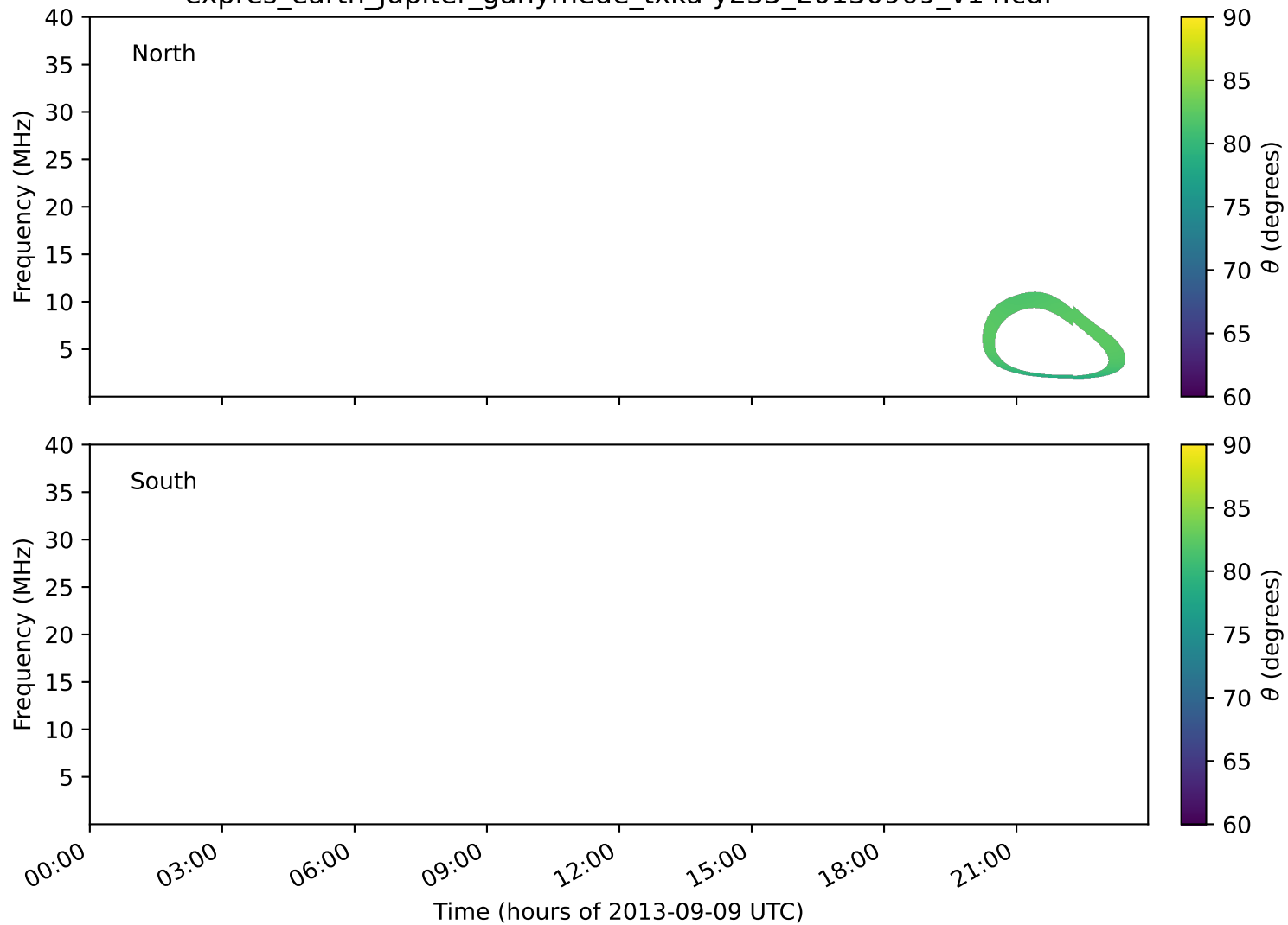
expres_earth_jupiter_ganymede_txka-y235_20130909_v14.cdf
