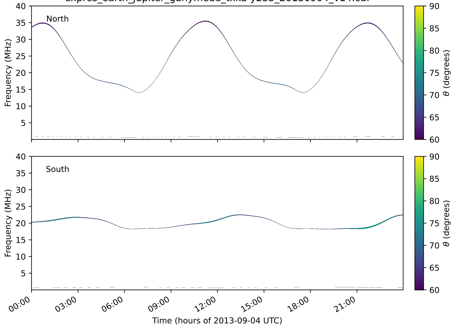
expres_earth_jupiter_ganymede_txka-y235_20130904_v14.cdf
