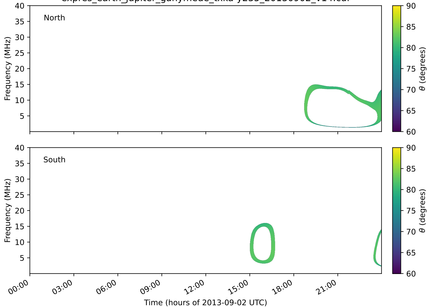
expres_earth_jupiter_ganymede_txka-y235_20130902_v14.cdf
