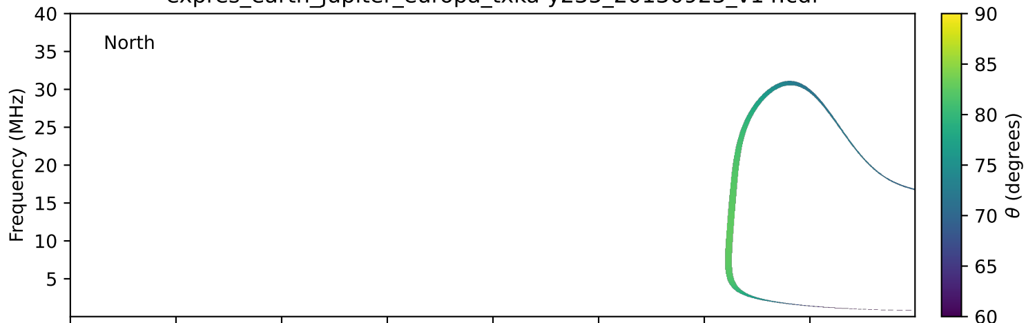
expres_earth_jupiter_europa_txka-y235_20130923_v14.cdf
