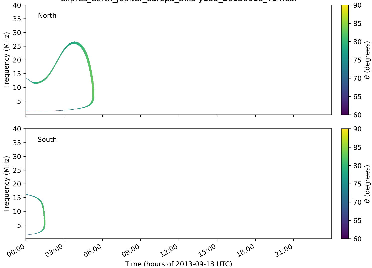
expres_earth_jupiter_europa_txka-y235_20130918_v14.cdf
