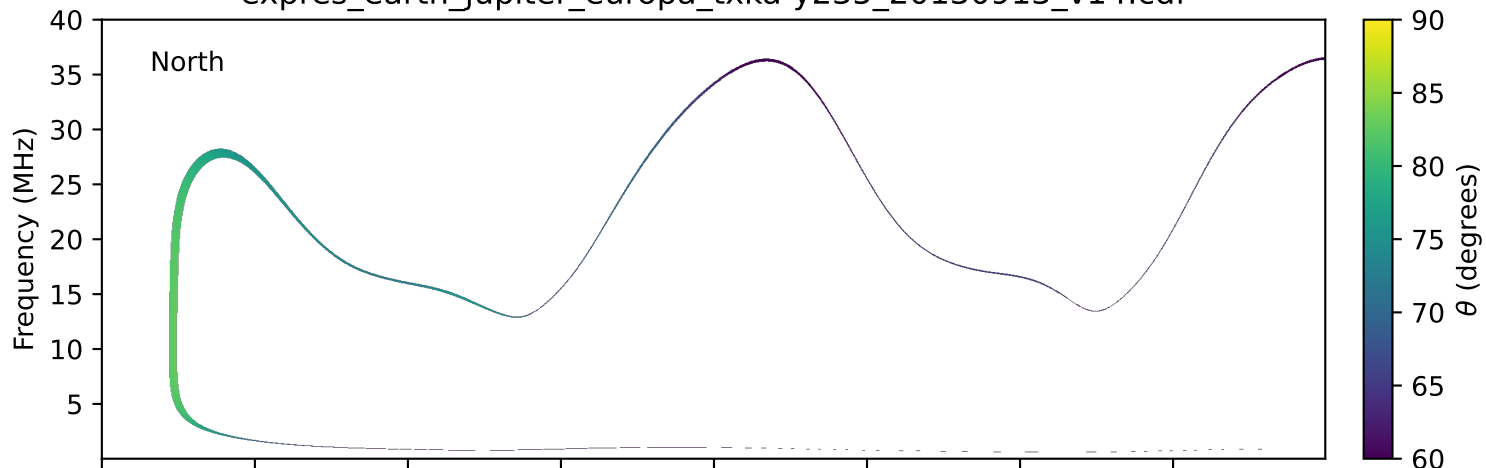
expres_earth_jupiter_europa_txka-y235_20130913_v14.cdf
