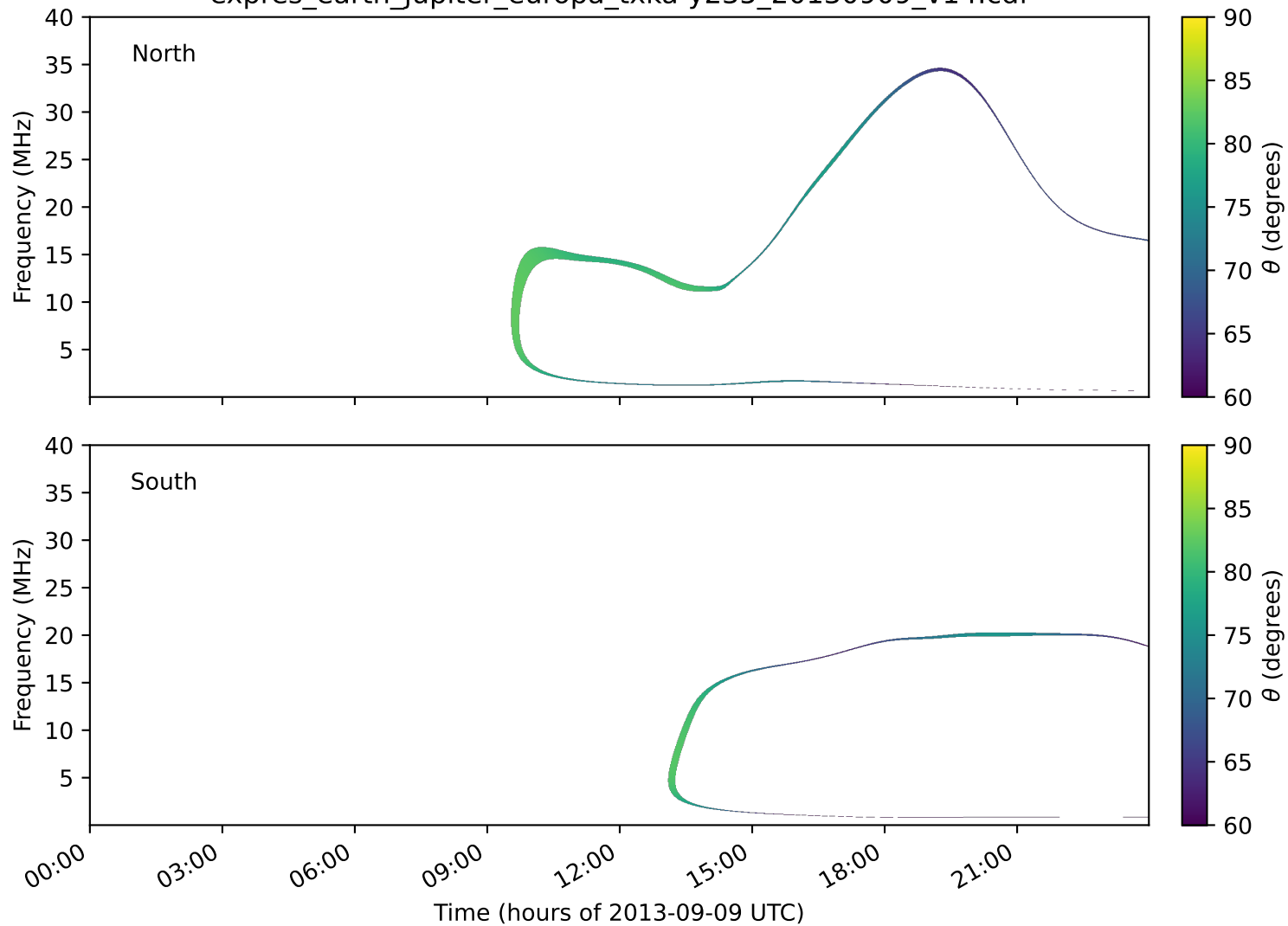
expres_earth_jupiter_europa_txka-y235_20130909_v14.cdf
