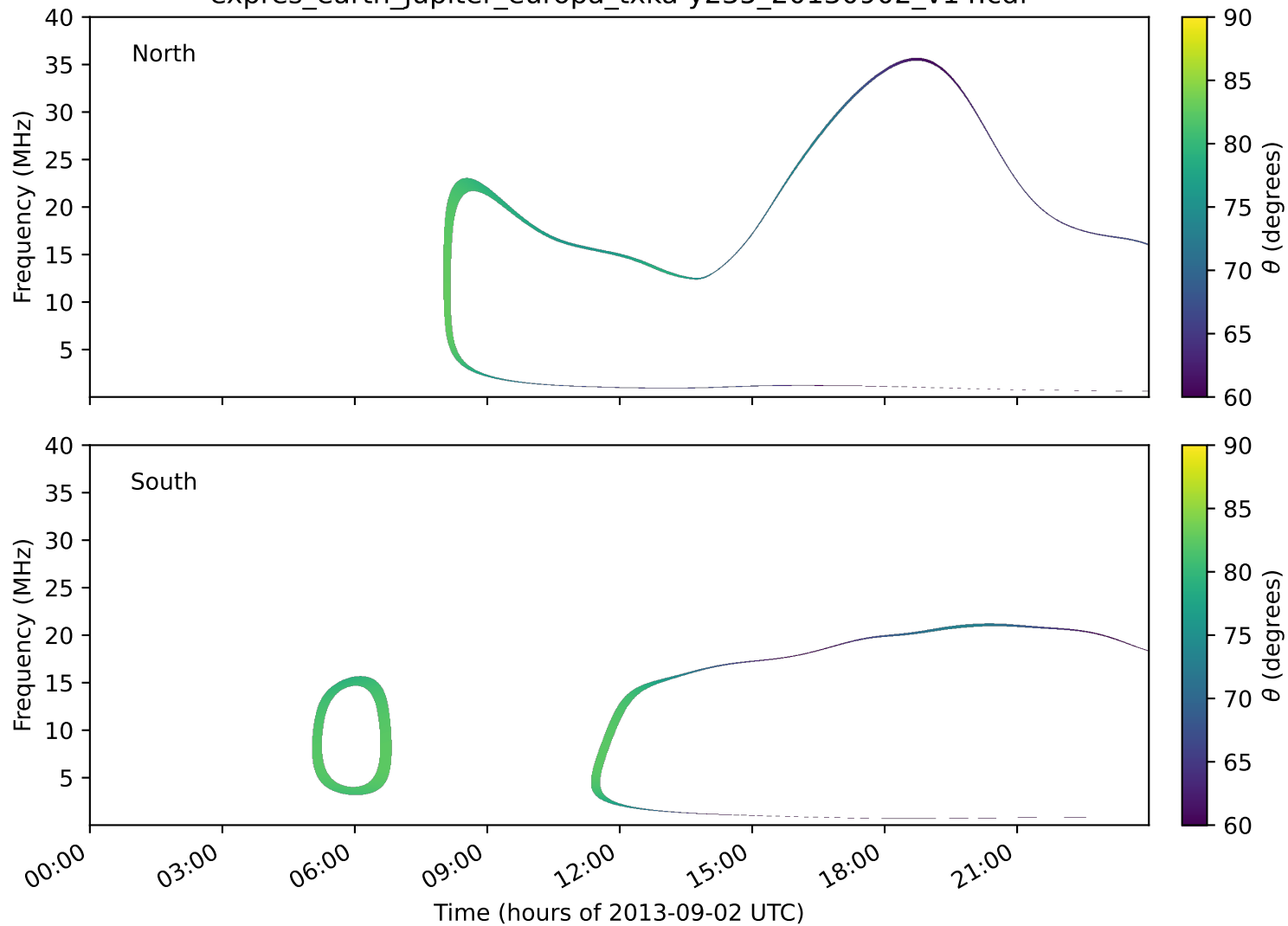
expres_earth_jupiter_europa_txka-y235_20130902_v14.cdf
