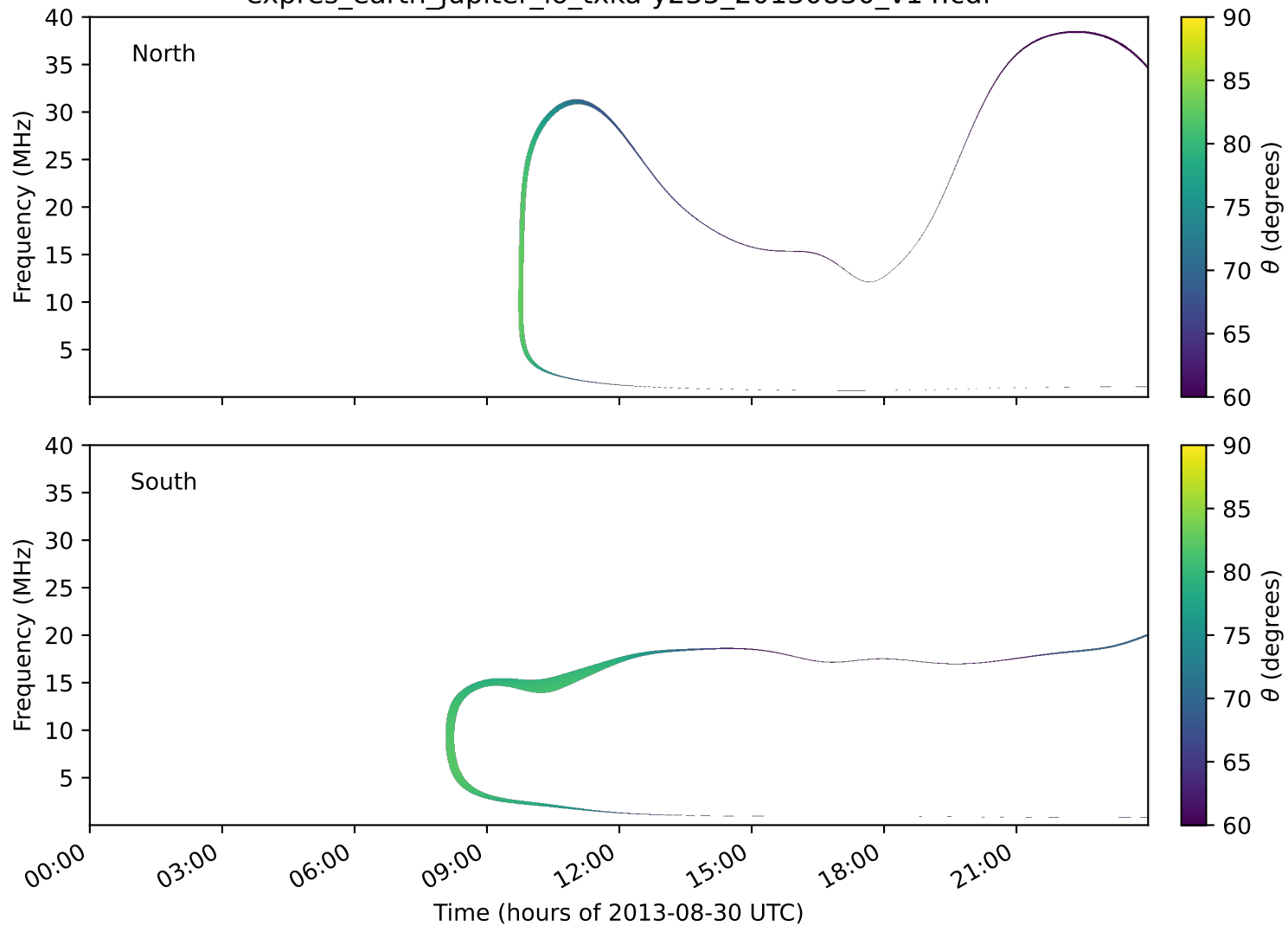
expres_earth_jupiter_io_txka-y235_20130830_v14.cdf
