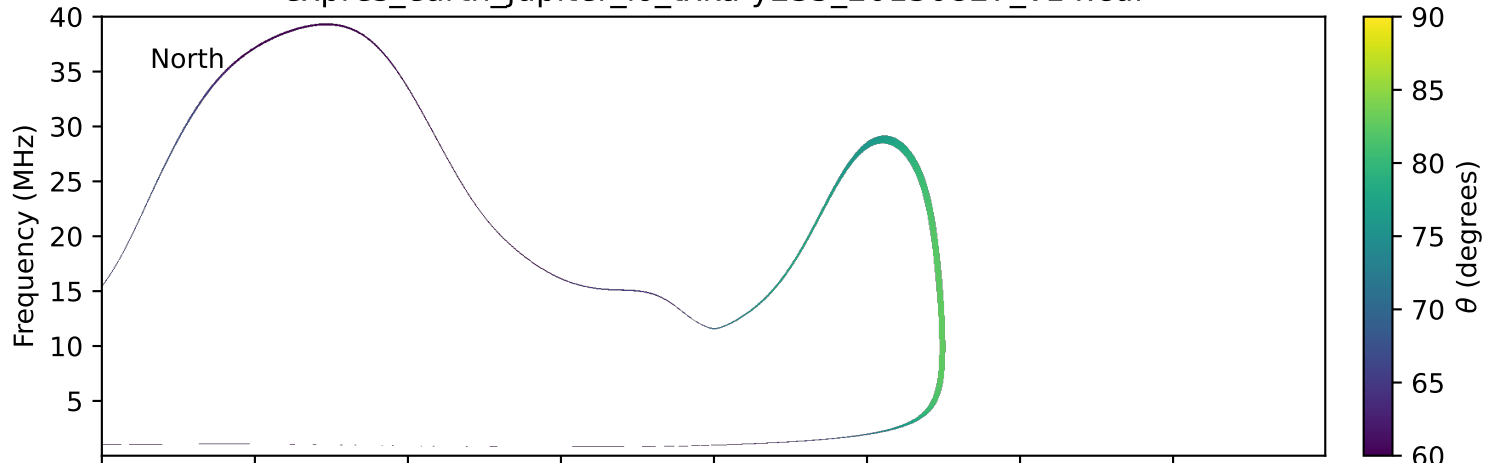
expres_earth_jupiter_io_txka-y235_20130827_v14.cdf
