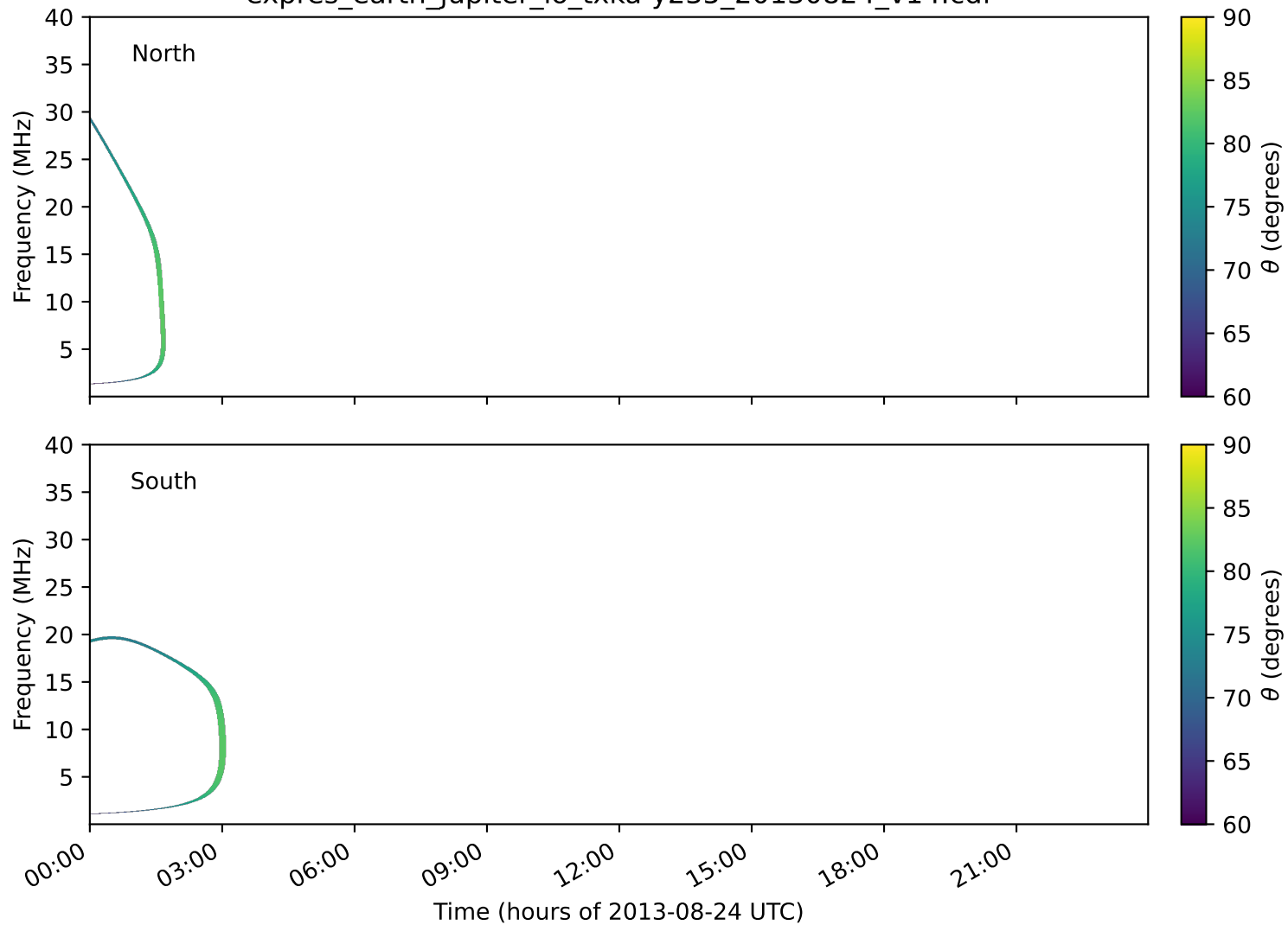
expres_earth_jupiter_io_txka-y235_20130824_v14.cdf
