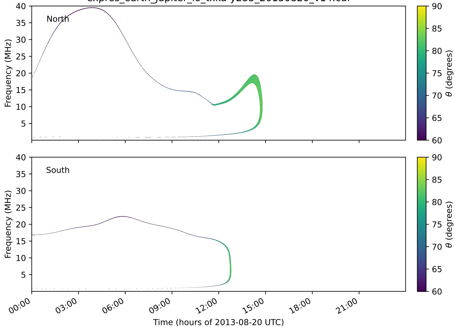
expres_earth_jupiter_io_txka-y235_20130820_v14.cdf
