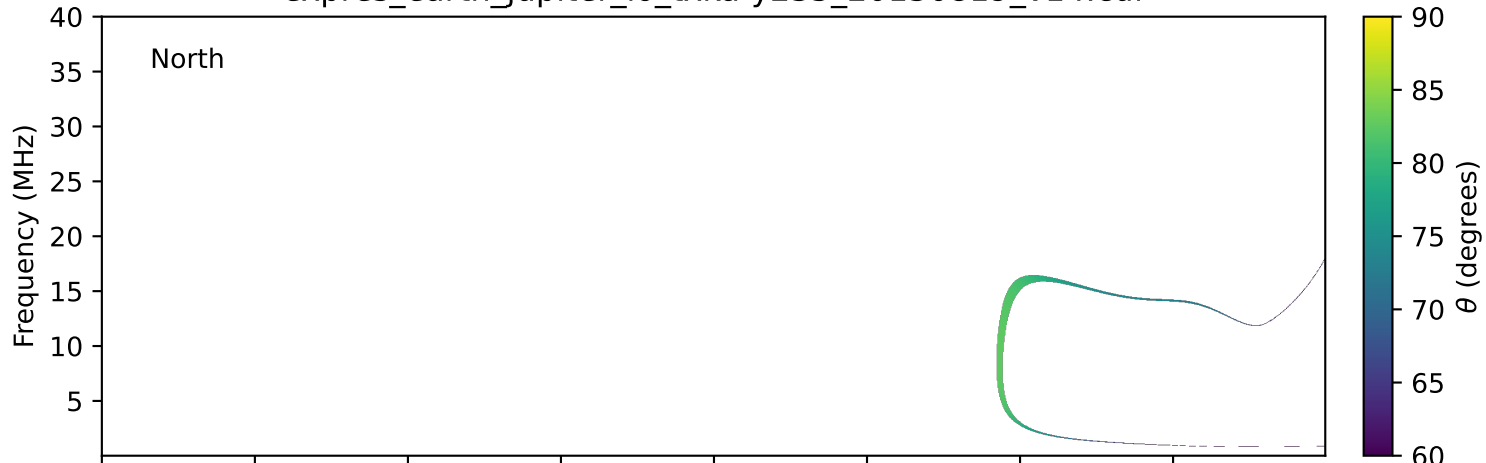
expres_earth_jupiter_io_txka-y235_20130819_v14.cdf
