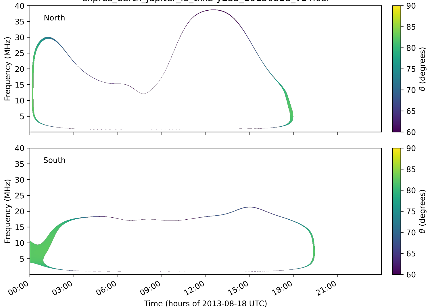
expres_earth_jupiter_io_txka-y235_20130818_v14.cdf
