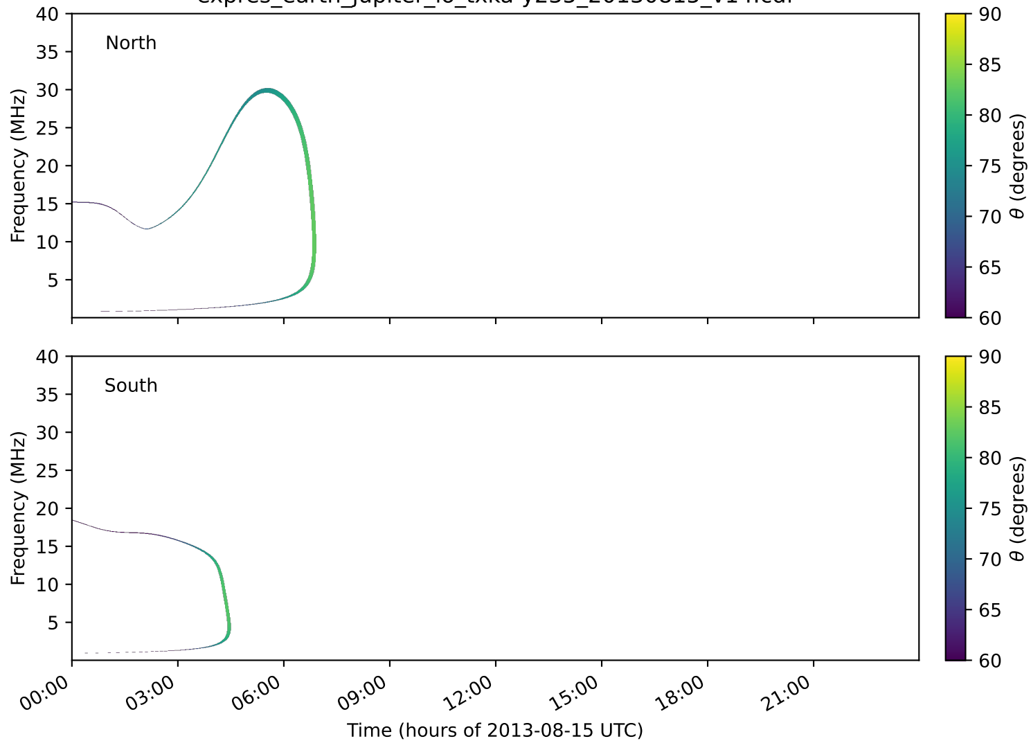
expres_earth_jupiter_io_txka-y235_20130815_v14.cdf
