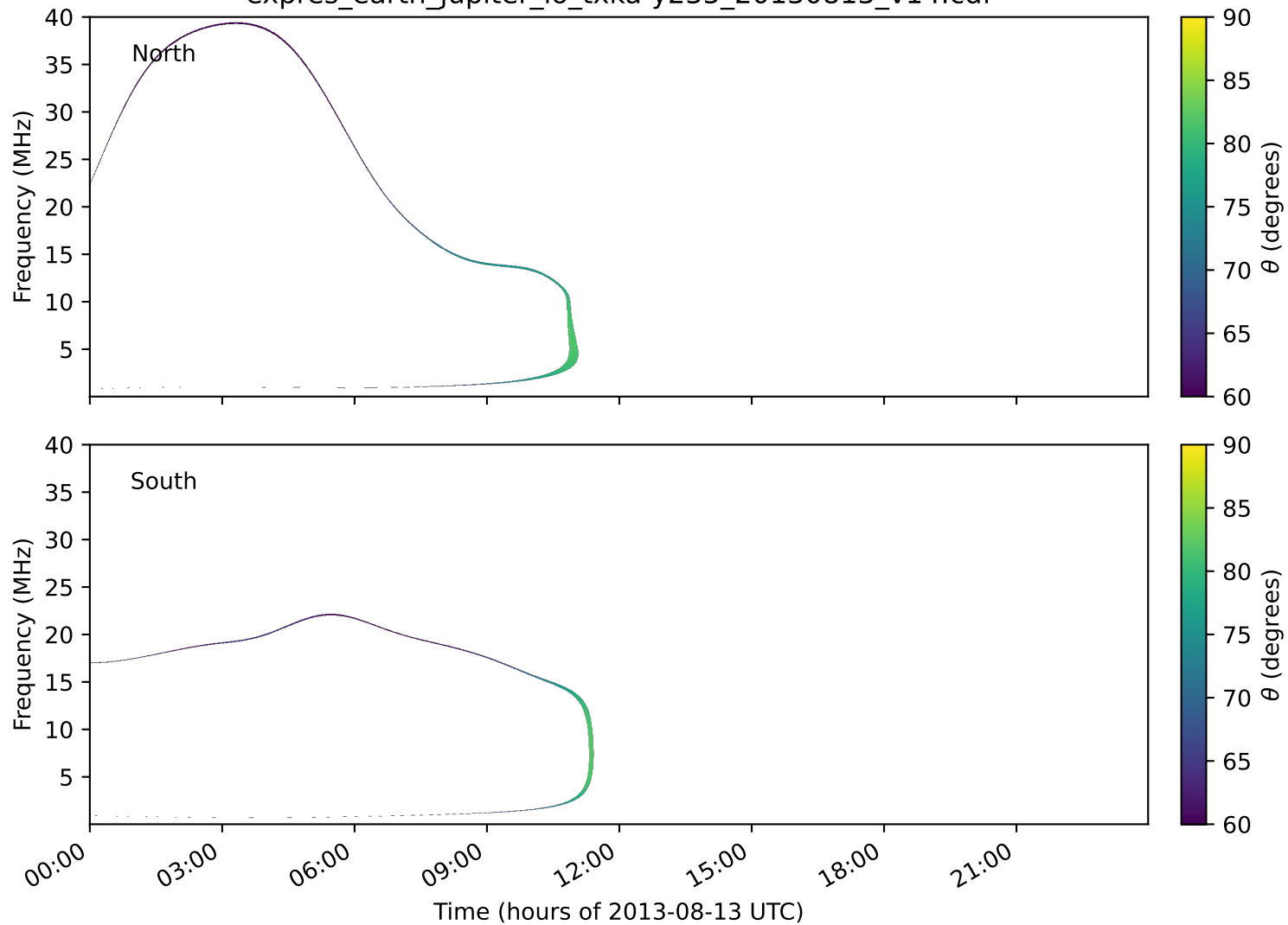
expres_earth_jupiter_io_txka-y235_20130813_v14.cdf
