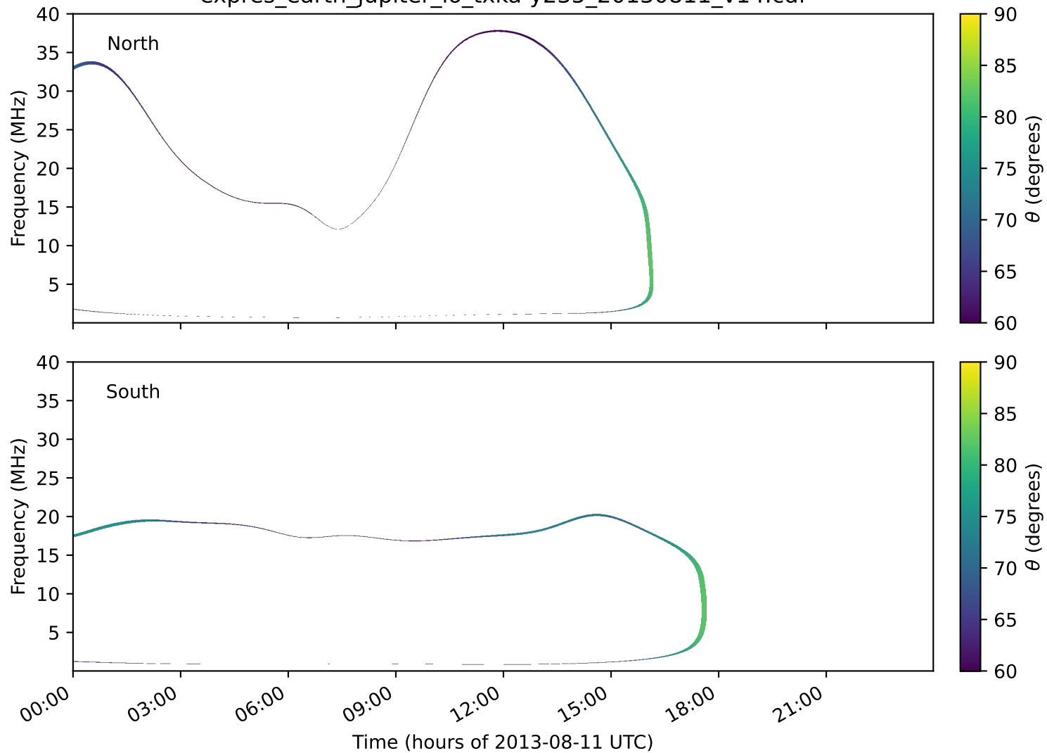
expres_earth_jupiter_io_txka-y235_20130811_v14.cdf
