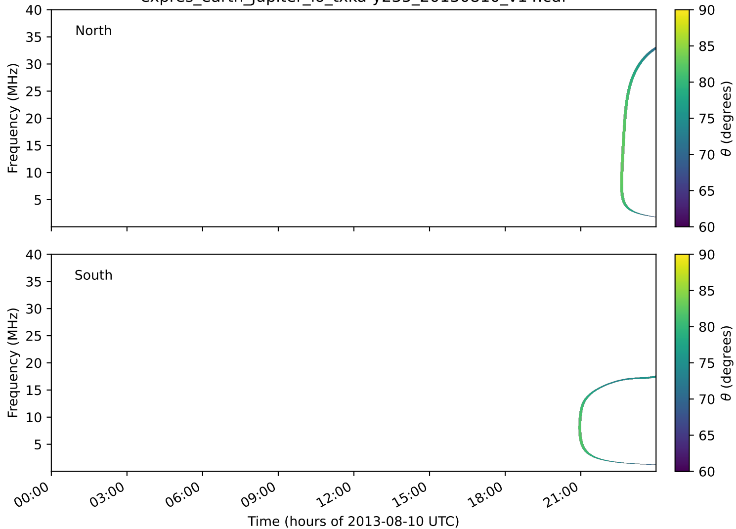
expres_earth_jupiter_io_txka-y235_20130810_v14.cdf
