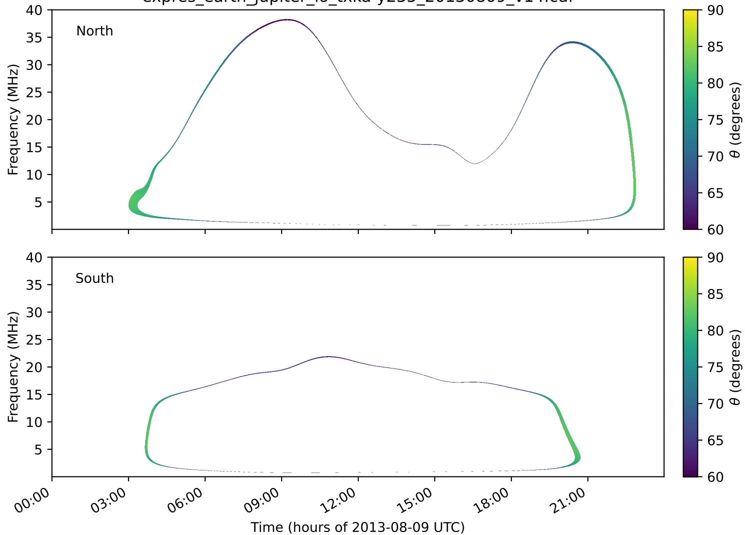
expres_earth_jupiter_io_txka-y235_20130809_v14.cdf
