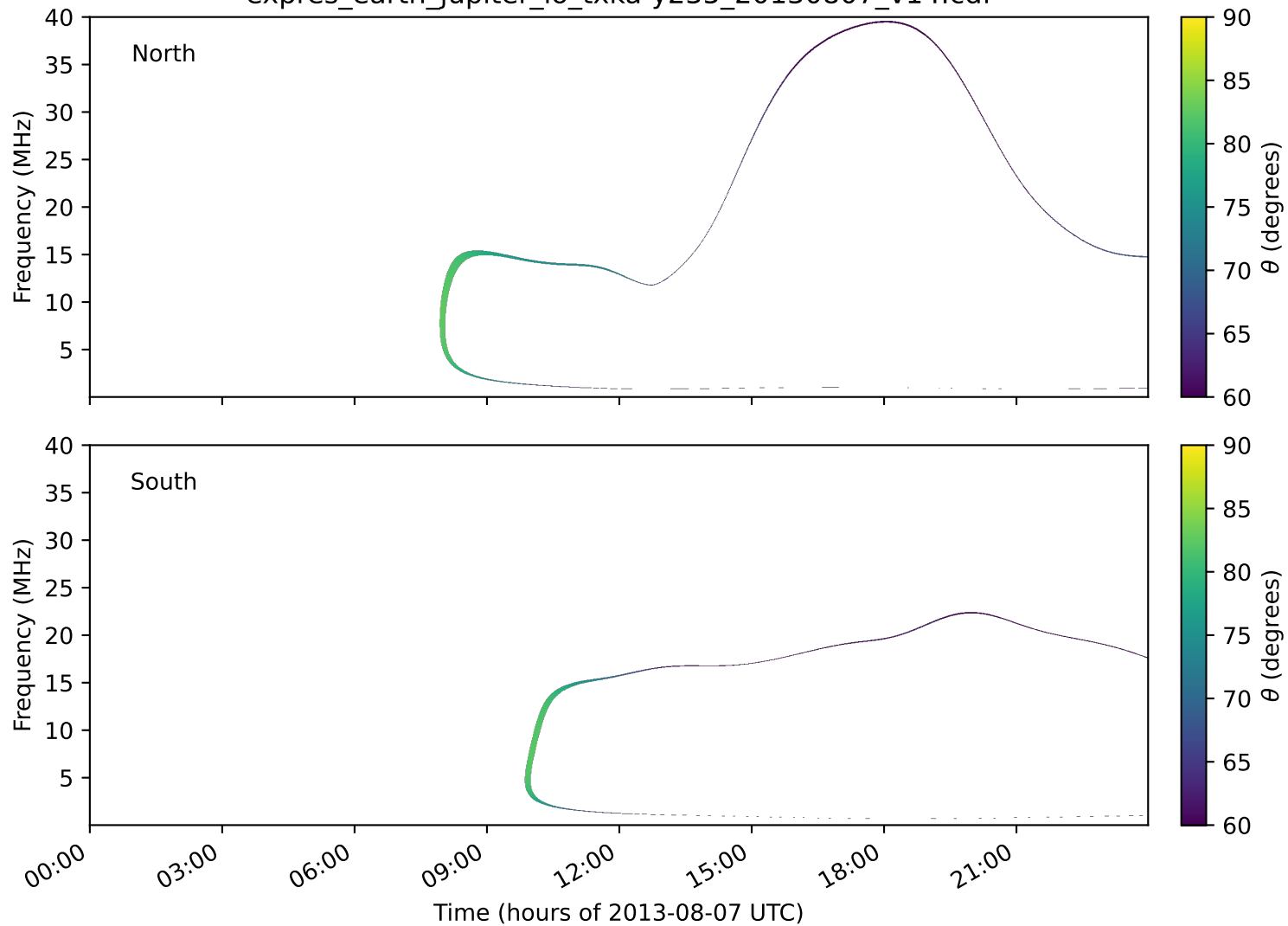
expres_earth_jupiter_io_txka-y235_20130807_v14.cdf
