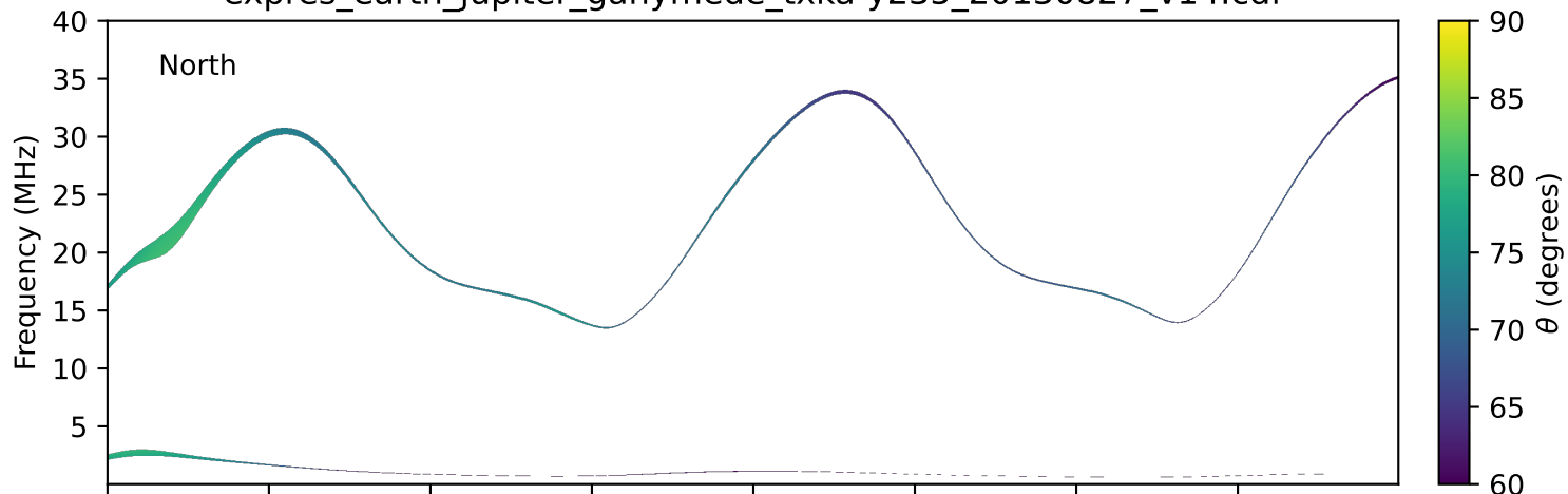
expres_earth_jupiter_ganymede_txka-y235_20130827_v14.cdf
