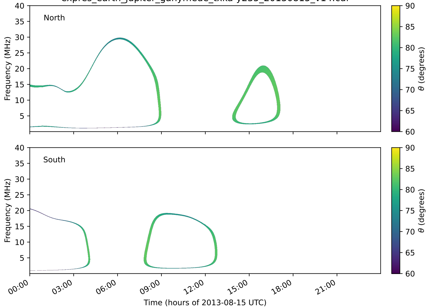
expres_earth_jupiter_ganymede_txka-y235_20130815_v14.cdf
