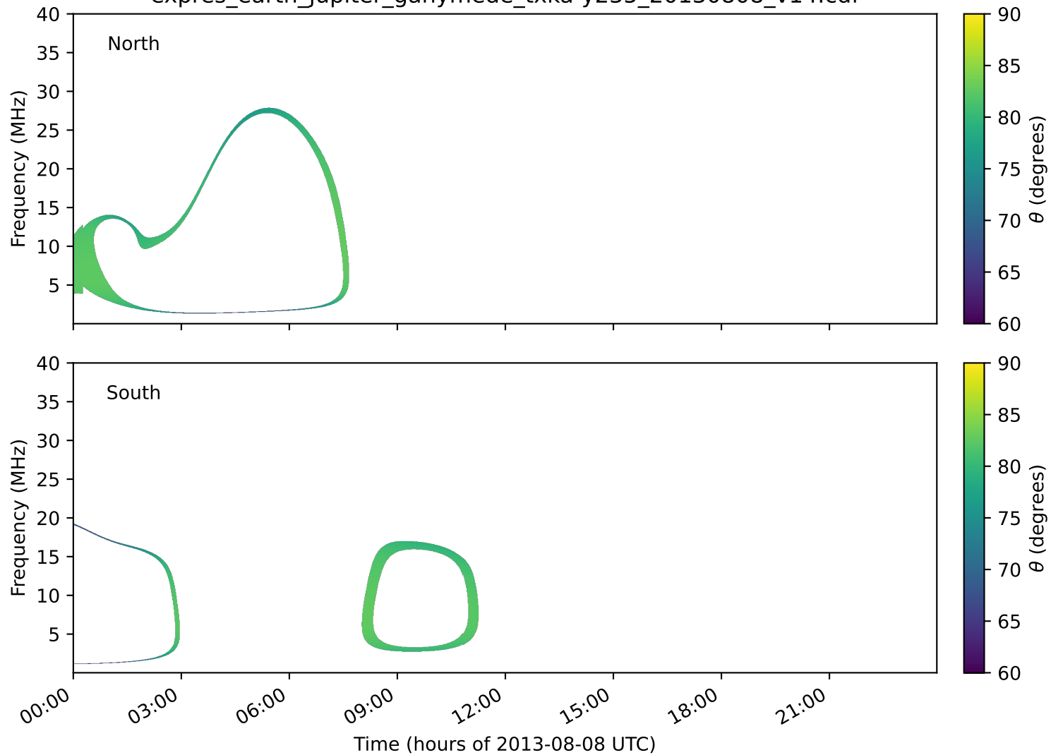
expres_earth_jupiter_ganymede_txka-y235_20130808_v14.cdf
