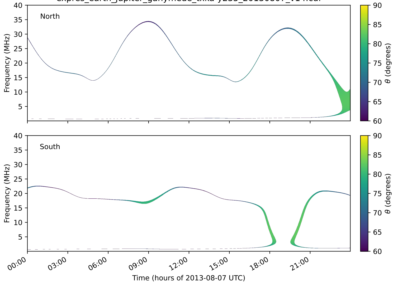
expres_earth_jupiter_ganymede_txka-y235_20130807_v14.cdf
