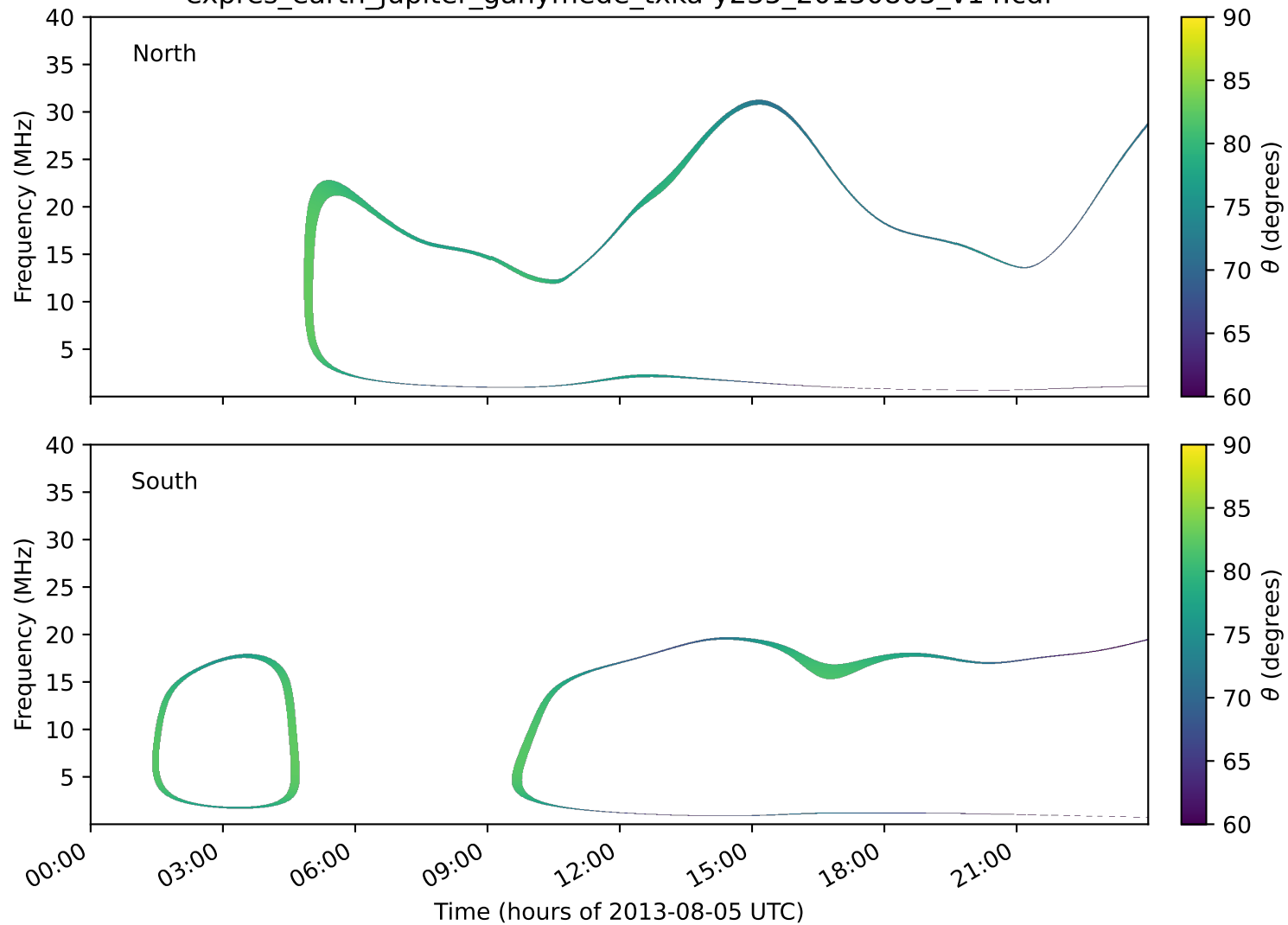
expres_earth_jupiter_ganymede_txka-y235_20130805_v14.cdf
