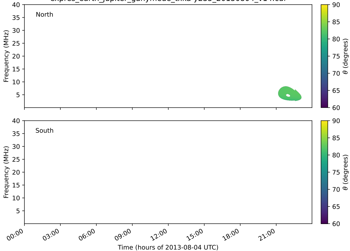
expres_earth_jupiter_ganymede_txka-y235_20130804_v14.cdf
