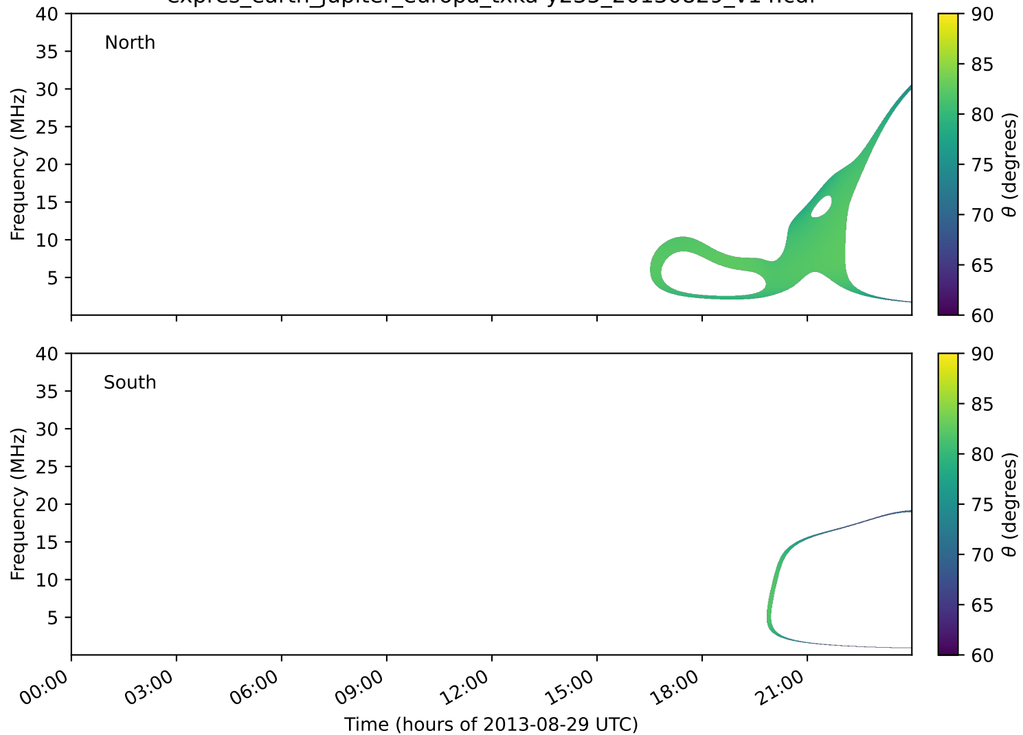
expres_earth_jupiter_europa_txka-y235_20130829_v14.cdf
