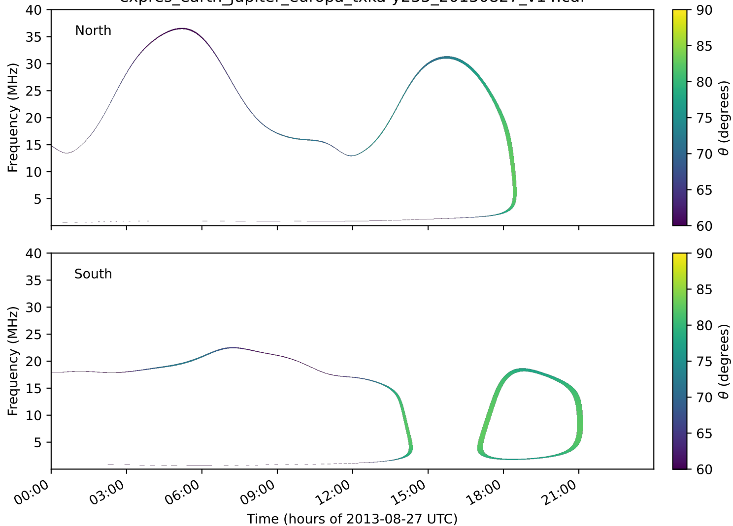
expres_earth_jupiter_europa_txka-y235_20130827_v14.cdf
