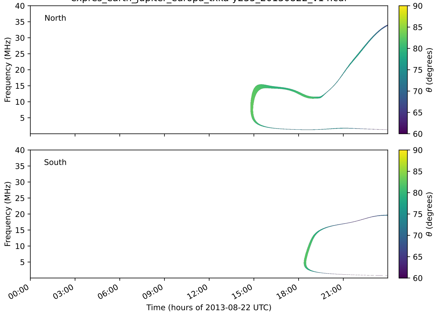
expres_earth_jupiter_europa_txka-y235_20130822_v14.cdf
