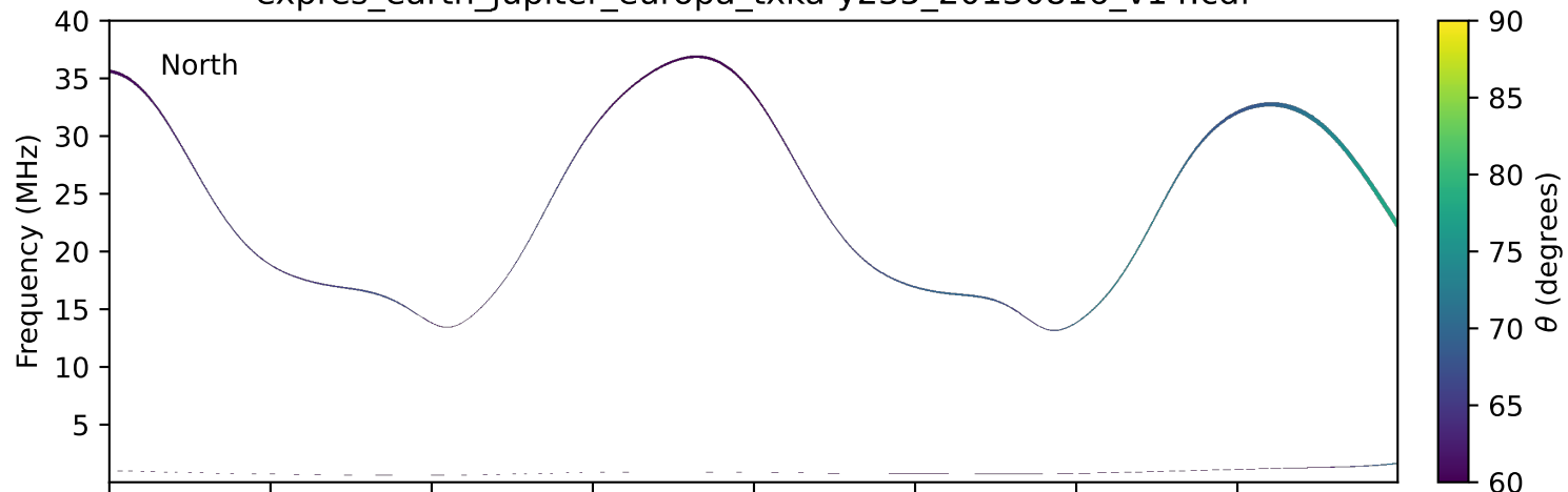
expres_earth_jupiter_europa_txka-y235_20130816_v14.cdf
