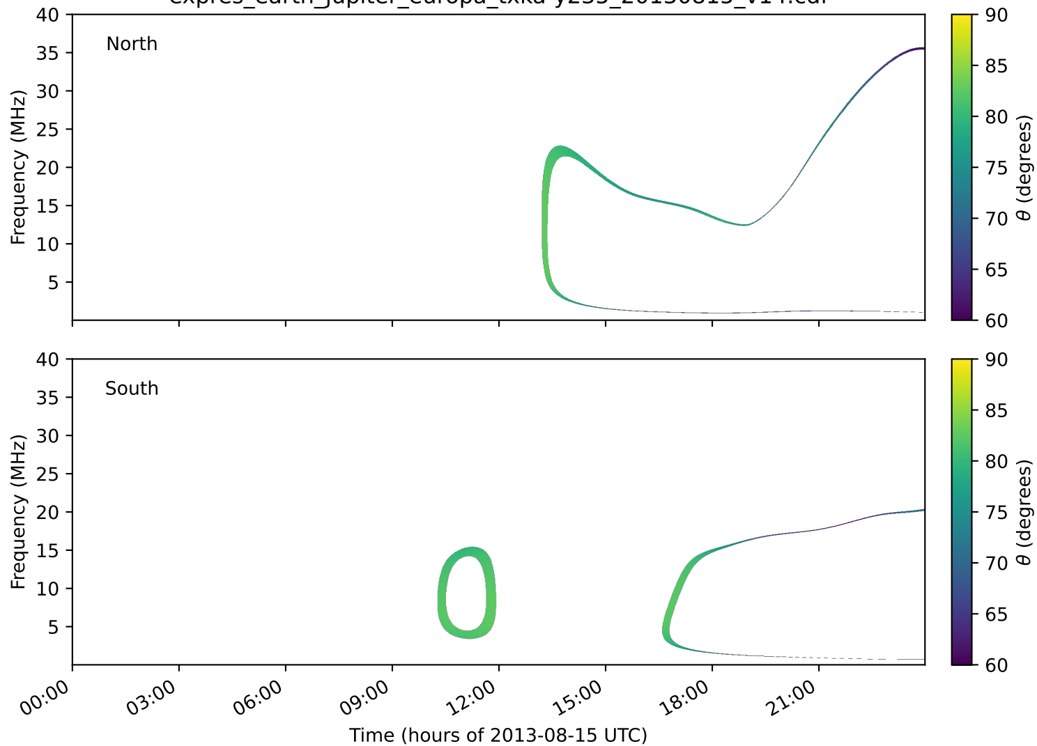
expres_earth_jupiter_europa_txka-y235_20130815_v14.cdf
