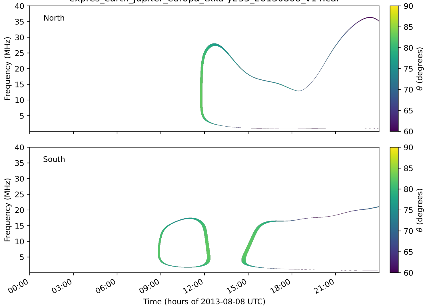
expres_earth_jupiter_europa_txka-y235_20130808_v14.cdf
